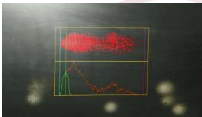
Figure 1: Cell with comet
