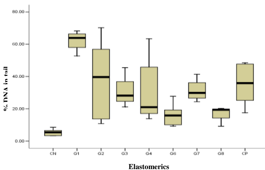
Graph 1: Box plots - Groups of elastomerics and proportions of DNA damage.
